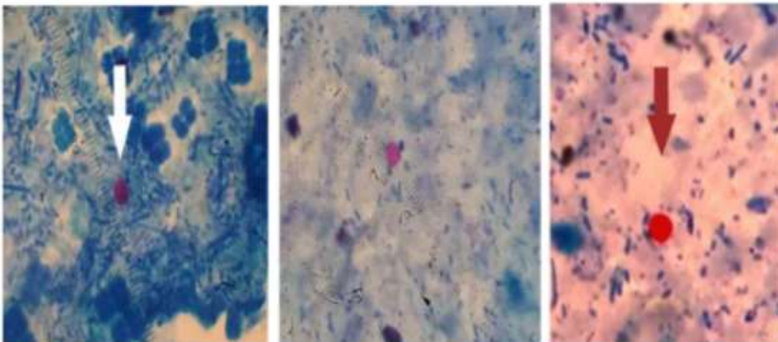
Figure 2. Microscopic image (100 high-power field) of Cryptosporidium oocysts (~5 µm) stained with the modified Ziehl-Neelsen stain technique.
