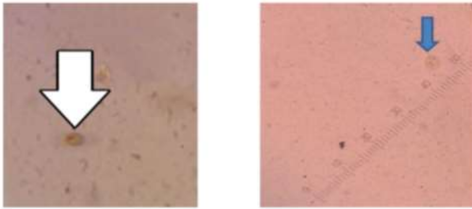
Figure 1. Microscopic image (100 high-power field) of Cryptosporidium oocysts (~5 µm) prepared from stool samples using the flotation technique.
